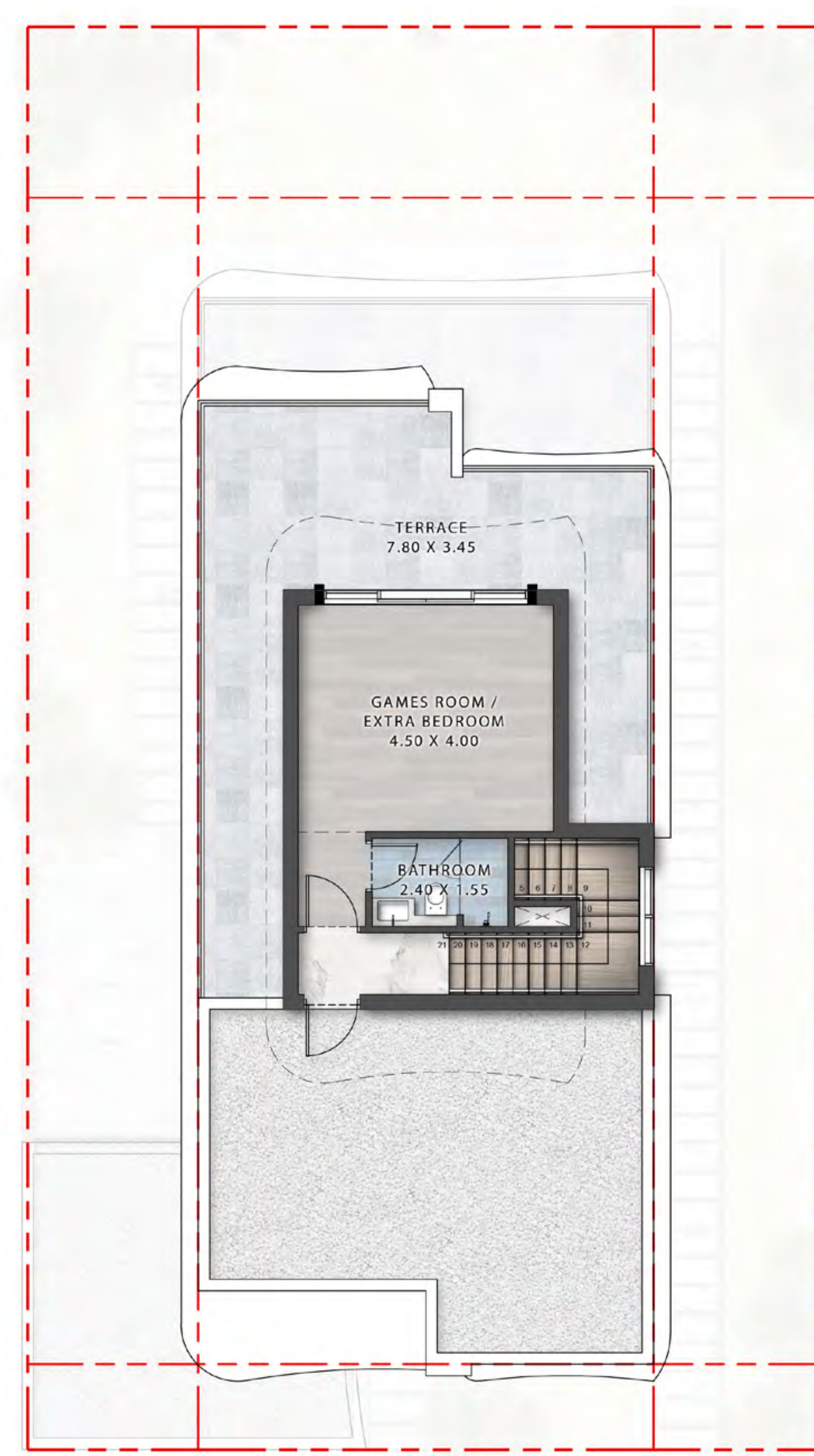
SECOND FLOOR
