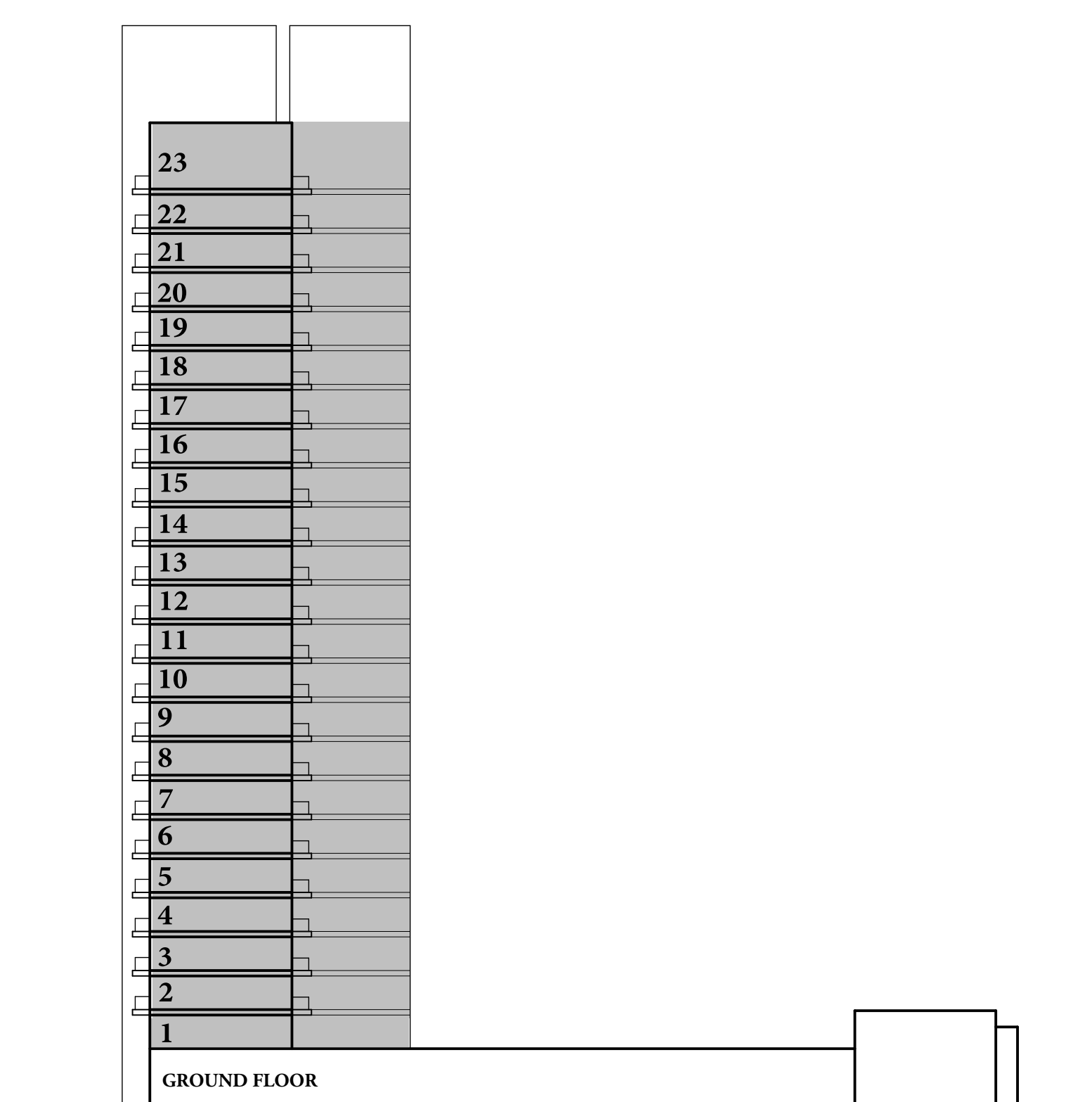
KEY SECTION
