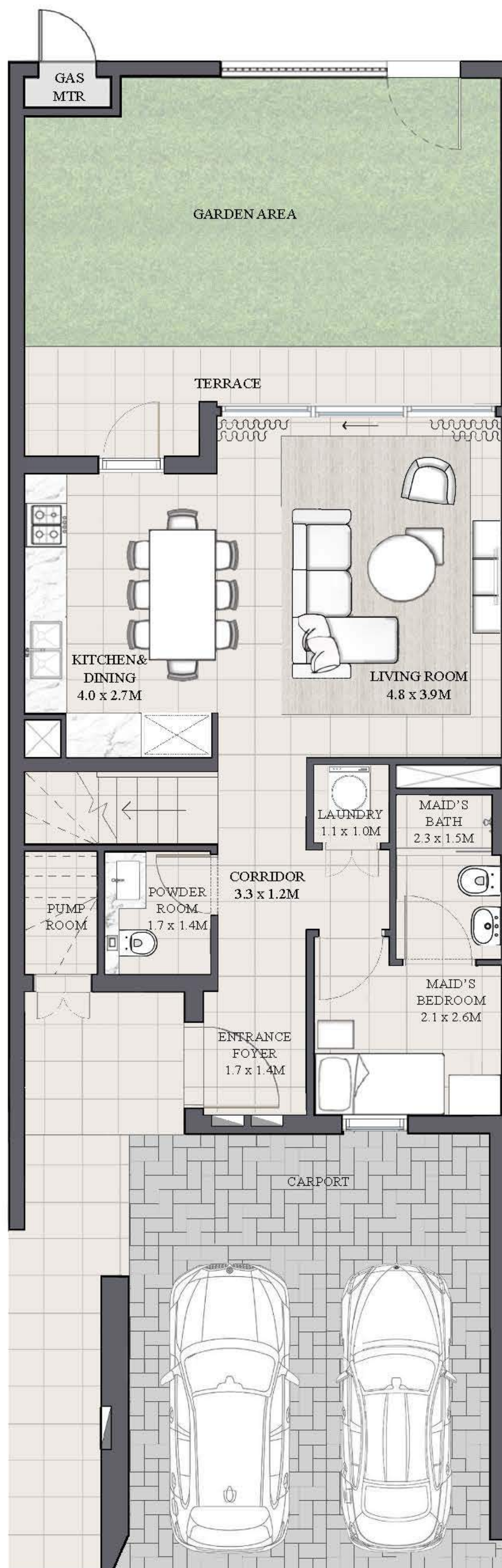
GROUND FLOOR
