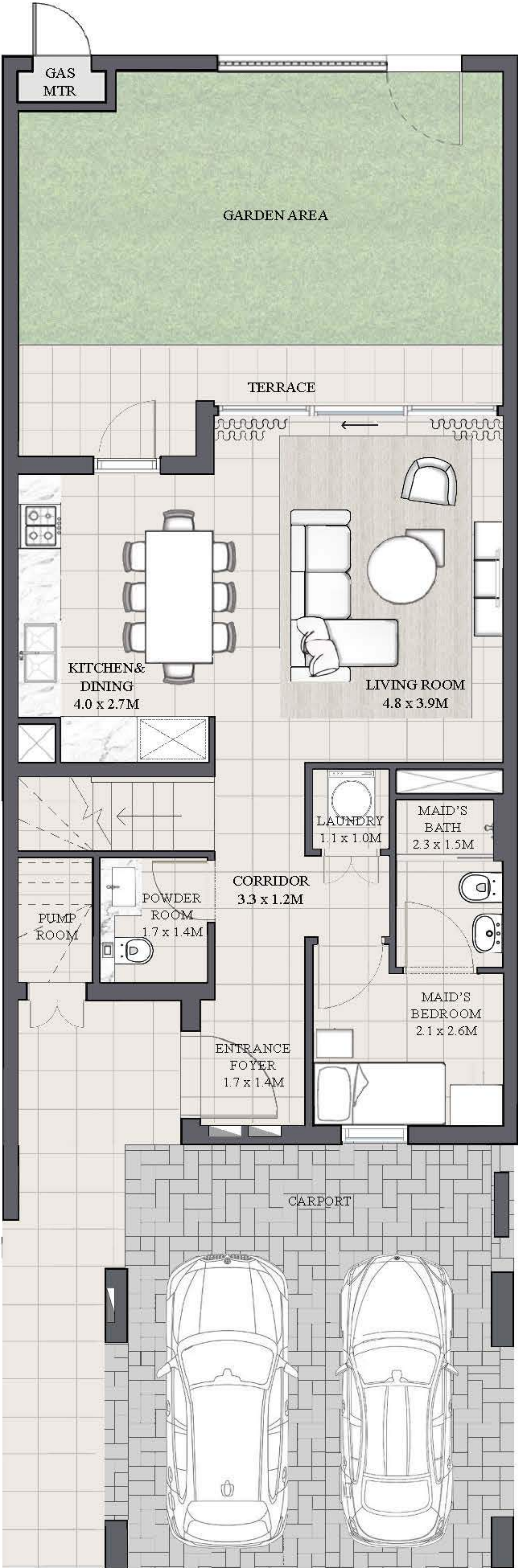
GROUND FLOOR
