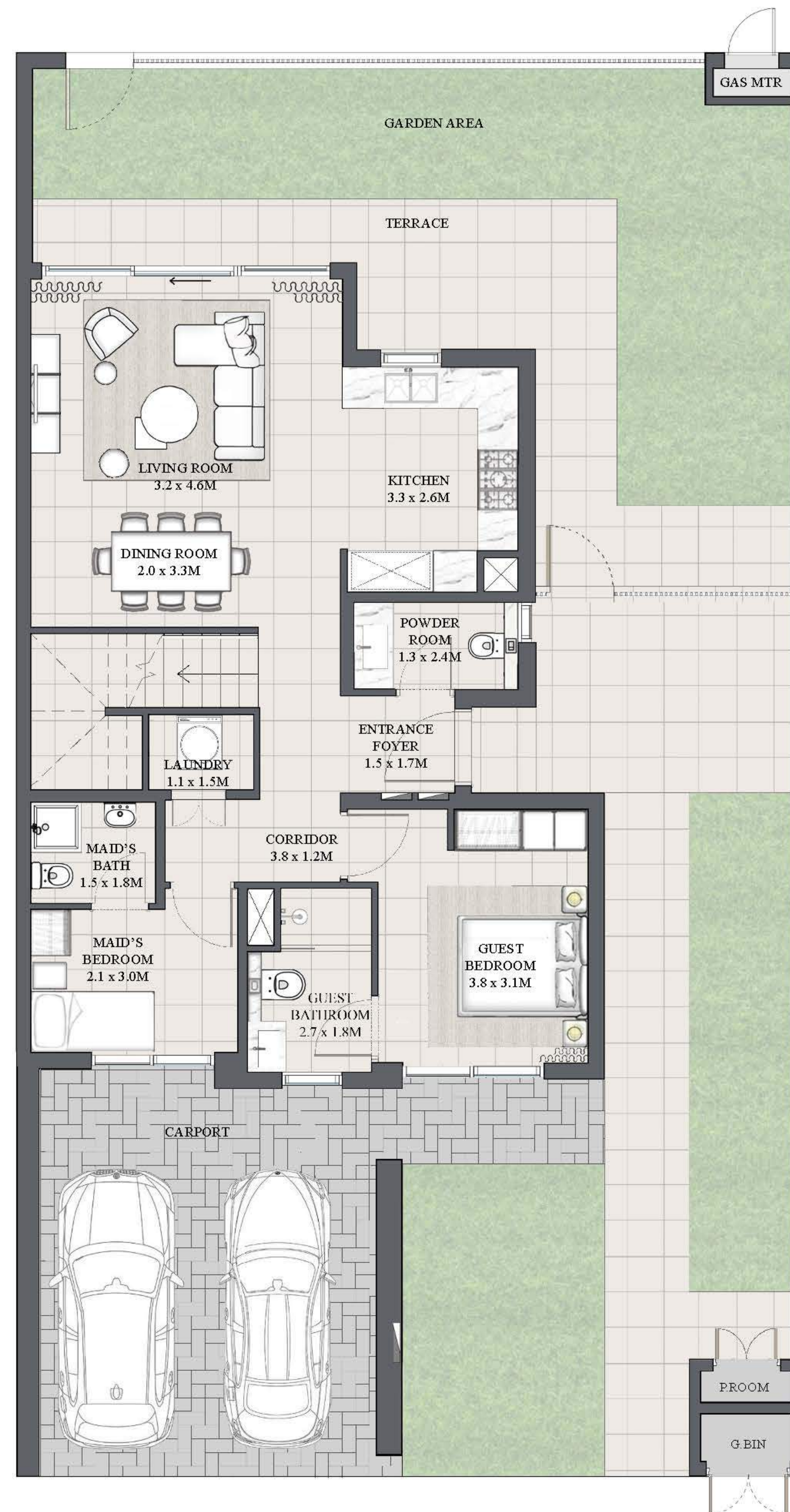
GROUND FLOOR
